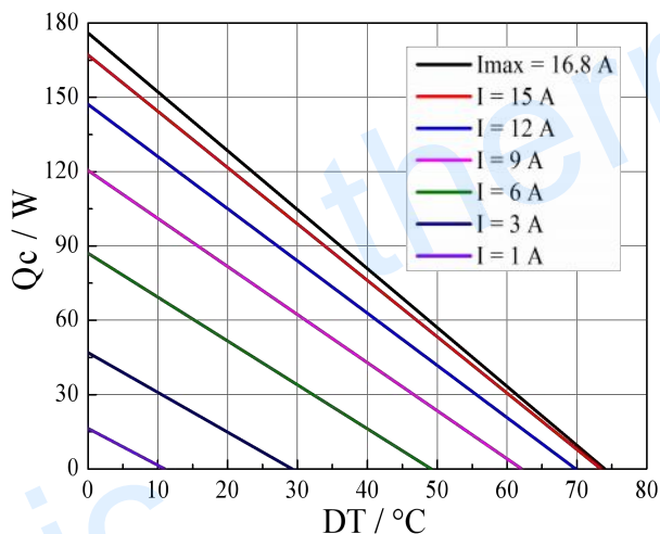
Performance Curves at T_h=27^\circ C
