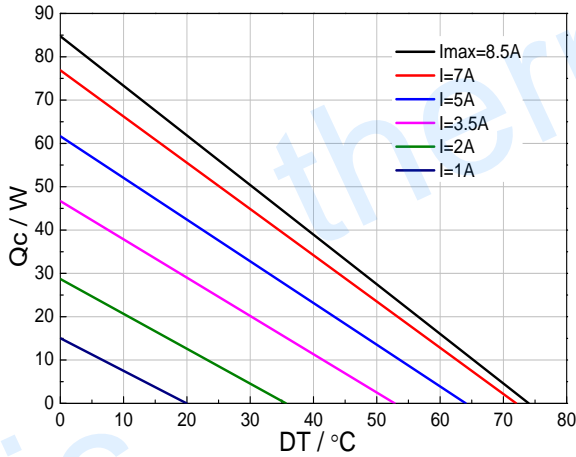
Performance Curves at T_h=27^\circ C
