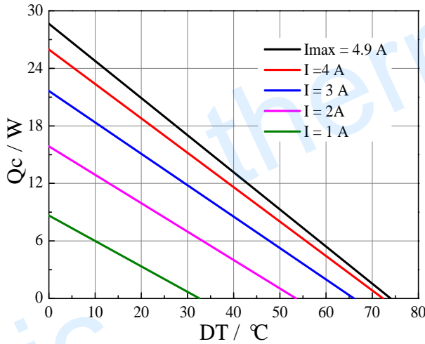
Performance Curves at T_h=25\text{ °C}
