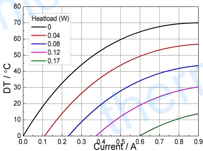
Standard Performance Graph ΔT= f(I)
