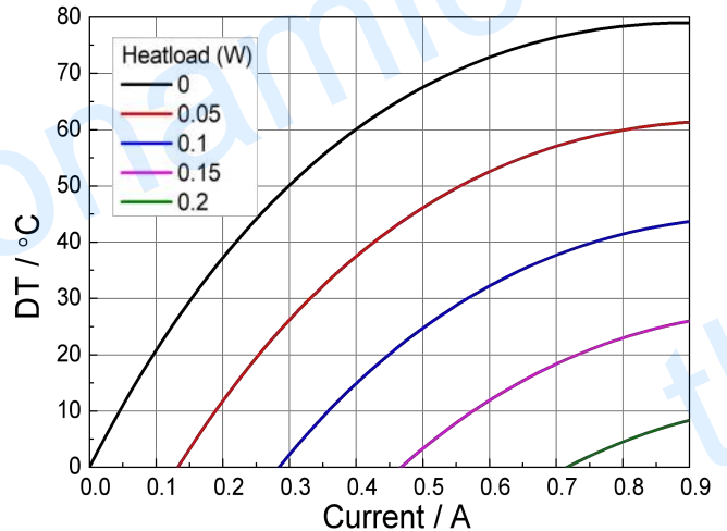
Standard Performance Graph ΔT= f(I)
