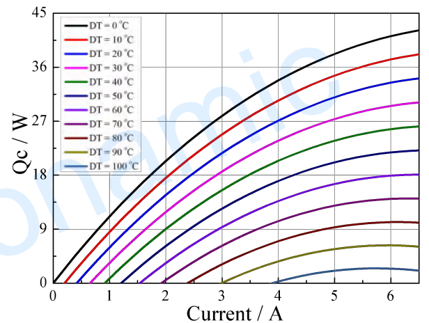
Standard Performance Graph Q_c = f(I)
